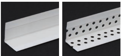
EU-27PT 27×2,500mm
